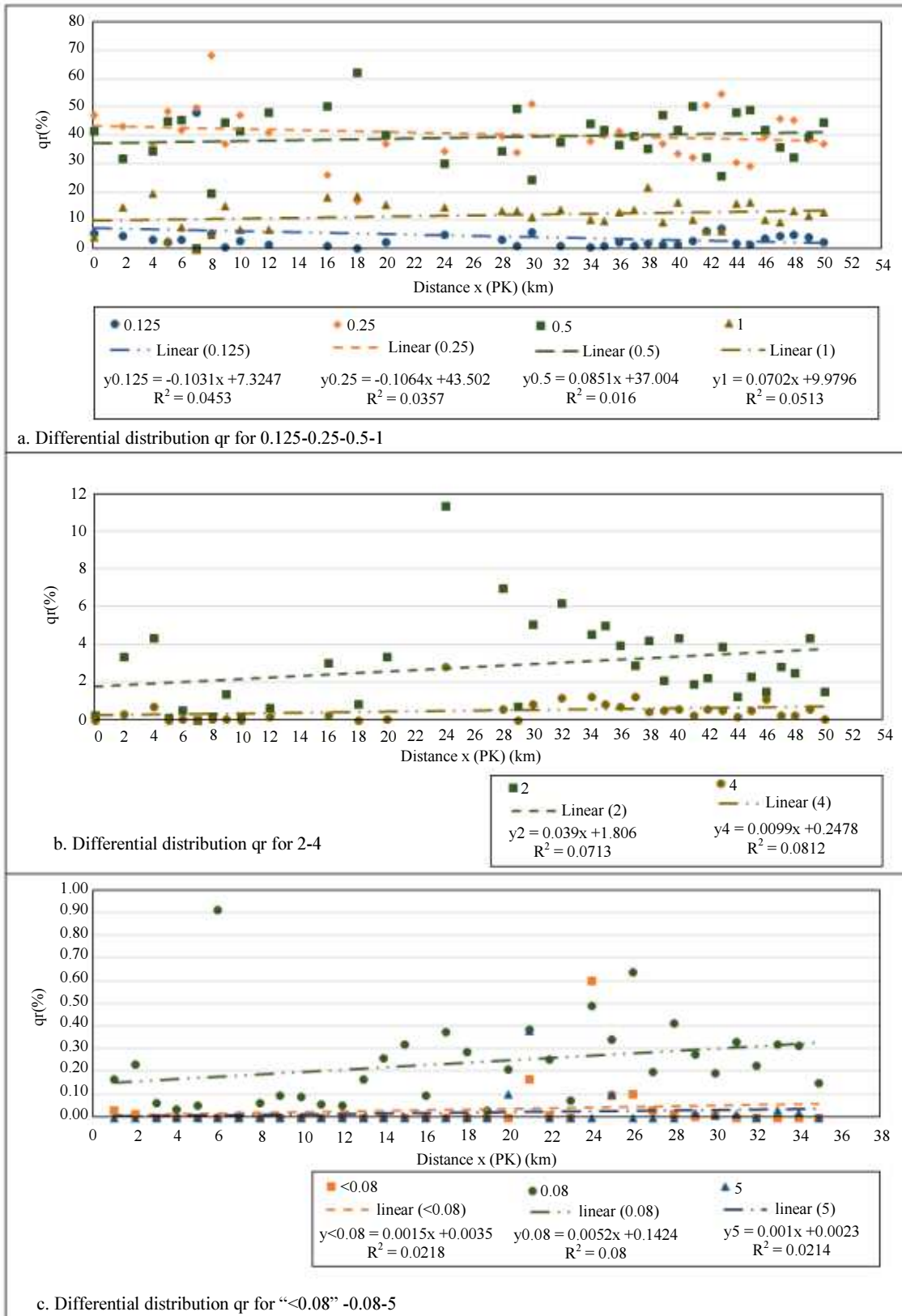
Fig. 5: Differential distributions of the particle size according to the profiles
