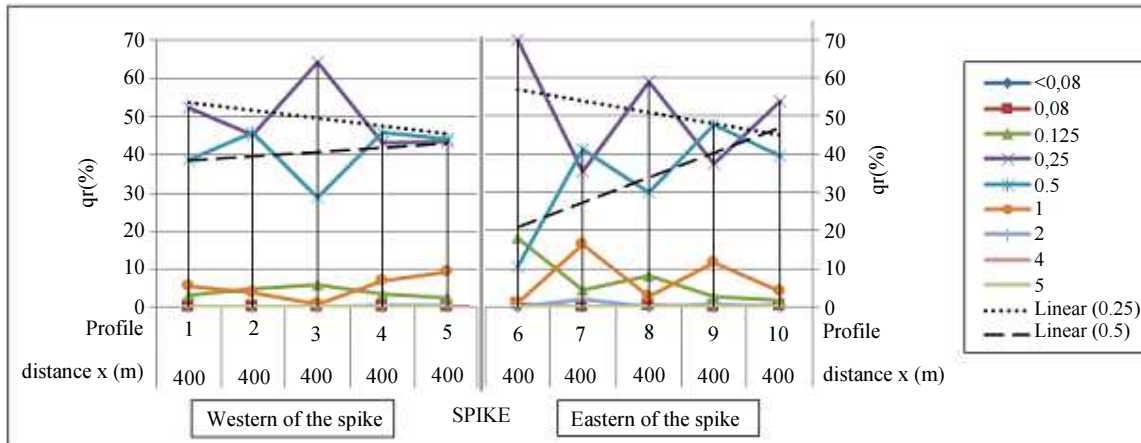
Fig. 6: Differential distributions of the grain size on each side of the spike E4
