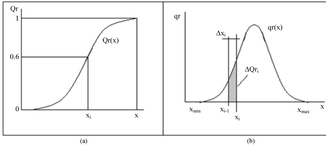
Fig. 1: Curves of cumulative and differential distributions (NF ISO 9276-1, 1998); (a) Cumulative distribution Qr(x) ; (b) Differential distribution qr(x)
