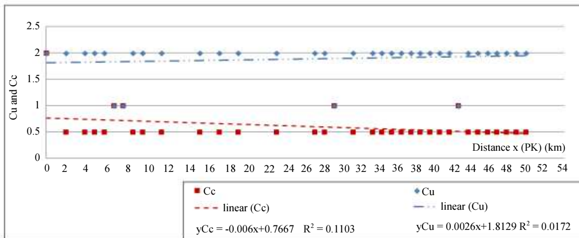
Fig. 7: Development of coefficients of uniformity ( C_u ) and of bending ( C_c ) according to profiles
