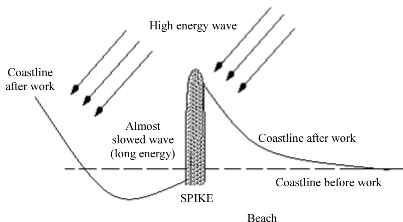
Fig. 11: Principle of sedimentary additions by waves at the level of spike E4
