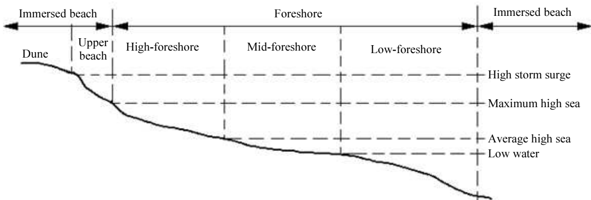
Fig. 3: Profile through a beach showing the foreshores and the aerial beach
