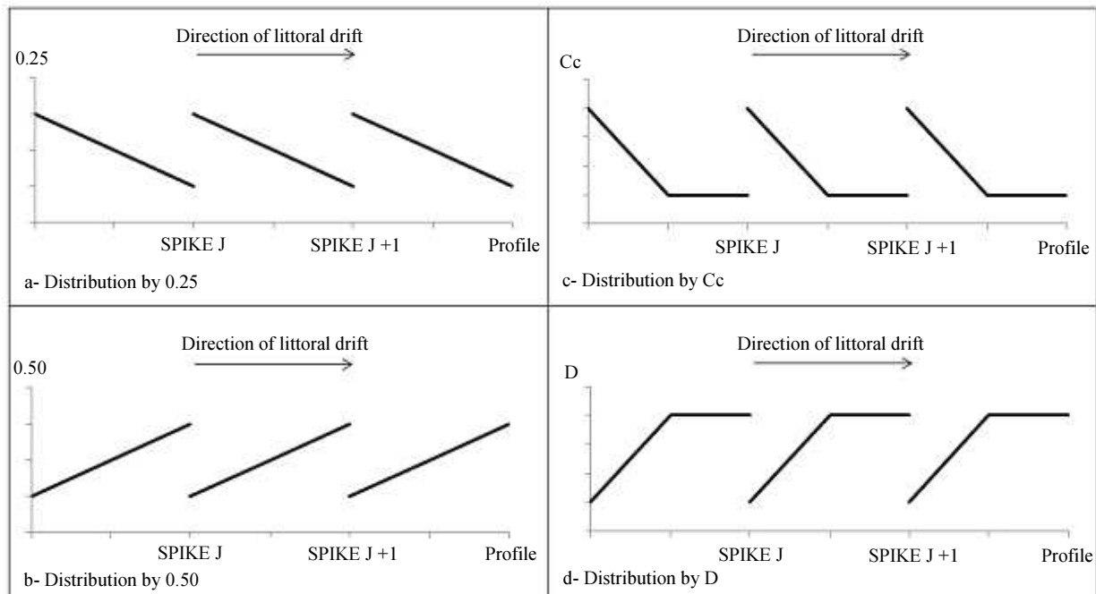
Fig. 12: Principle of distribution of sizes for a succession of the spike
